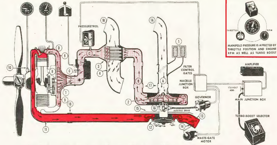
CIRCULAR DIAGRAM OF AN EXHAUST DRIVEN SUPERCHARGER ENGINE
