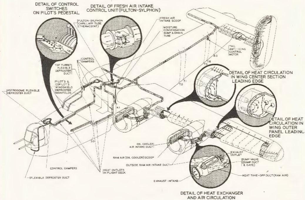
EXHAUST HEAT SYSTEM IN SOME LATE B-24'S
