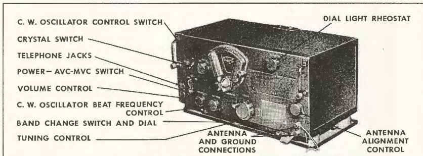
LIAISON RADIO RECEIVER
