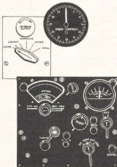
Radio Compass Controls
