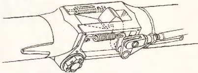
Down-Latch on Drag Strut Knuckle
