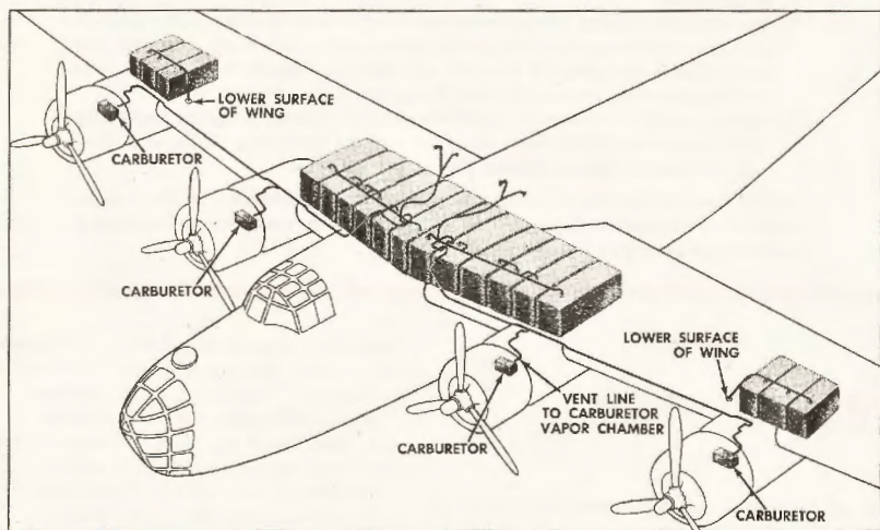
Fuel System
