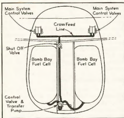
Bomb Bay Auxiliary Fuel System
