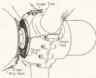
SLINGER RING DETAIL
